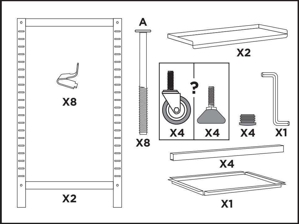
Frames & trolleys with shelves
